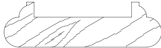
SCM 13002S 3/4 X 2-5/8
