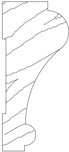
SCM 5015 1-1/8 X 2-1/2
