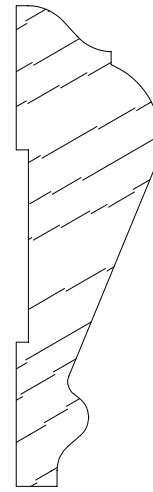
SCM 5014 3/4 X 2-1/2
