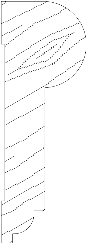
SCM 5042 1-1/2 X 4-1/4
