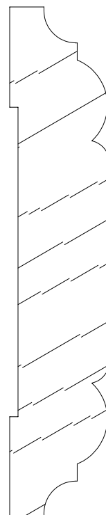
SCM 5033 3/4 X 3-13/16
