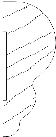
SCM 5002 7/8 X 2-1/4
