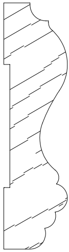
SCM 5012 5/8 X 2-1/2
