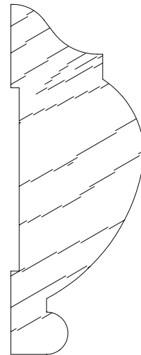
SCM 5050 1 X 2-5/8
