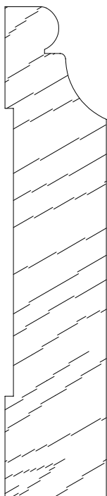
SCM 1112 3/4 X 3-5/8
