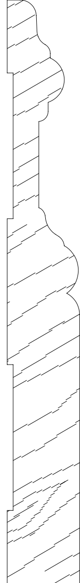
SCM 1130 3/4 X 6
