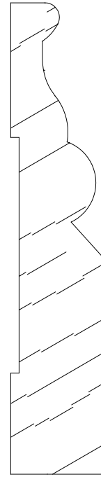
SCM 1020 3/4 X 3-7/8
