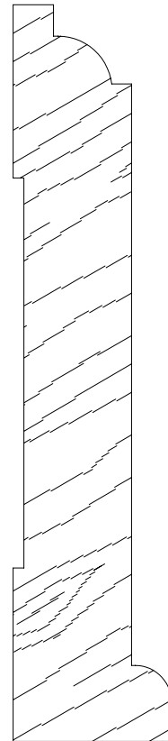
SCM 1101 15/16 X 3-1/4
