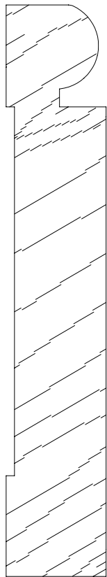
SCM 1089 3/4 X 4-1/4
