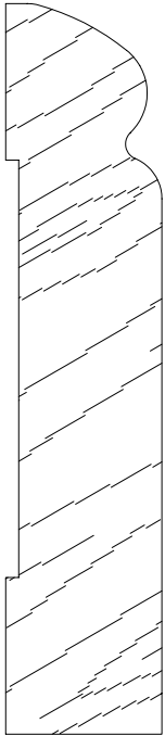
SCM 1032 3/4 X 3-1/2
