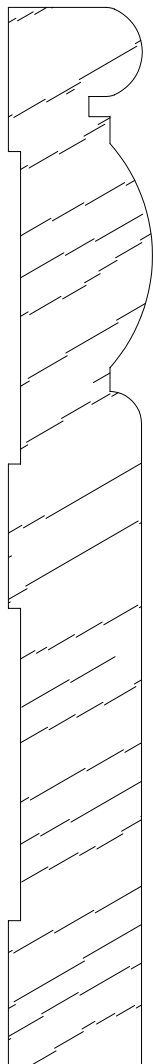
SCM 1138 3/4 X 5-1/2
