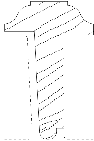
SCM 14003R 1-1/2 X 2-5/16
