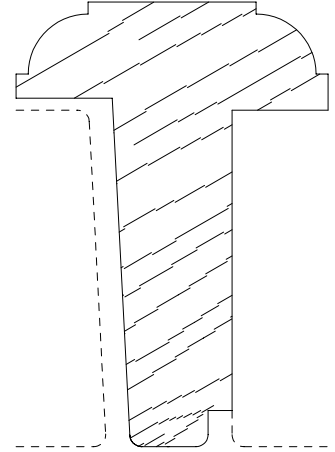
SCM 14002F 1-5/8 X 2-5/16
