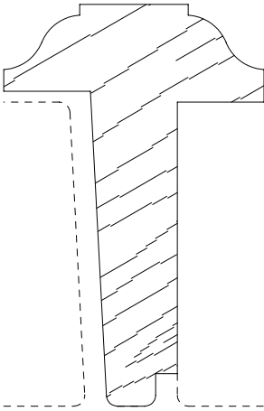
SCM 14003F 1-1/2 X 2-5/16
