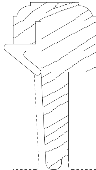
SCM 14005RW 1-1/2 X 3
