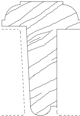
SCM 14002R 1-5/8 X 2-5/16
