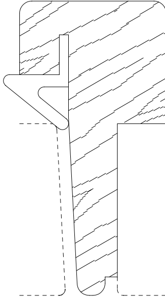
SCM 14004RW 1-1/2 X 3
